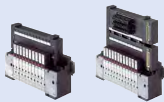
8640 Multipole or Fieldbus
