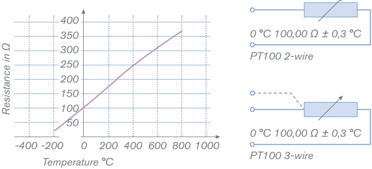
PT 100 resistance characteristic
